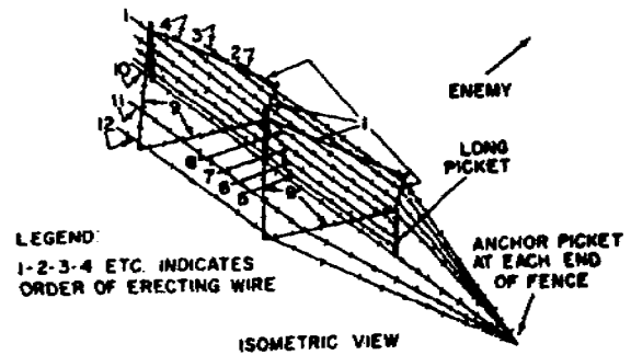
Figure 4-20. Double apron fence.
